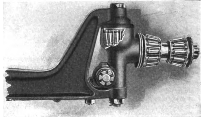
Front Axle with Timken Roller Bearing Knuckles.
